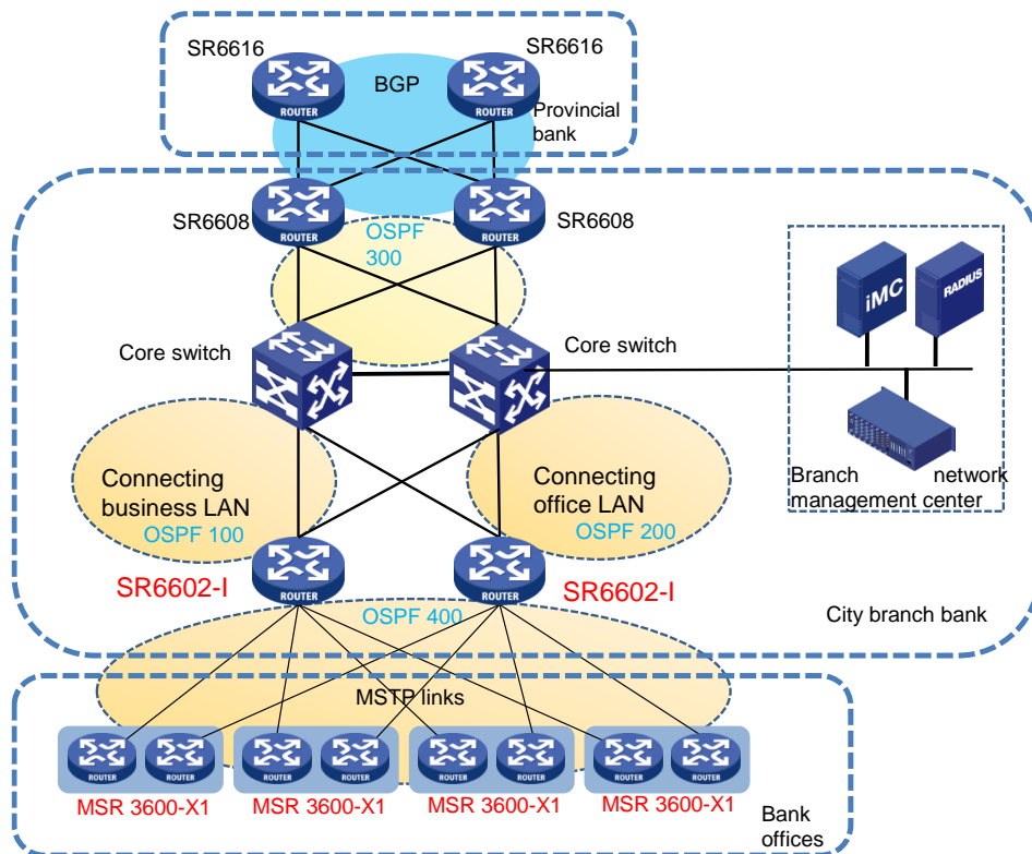
MSTP aggregation scenario
