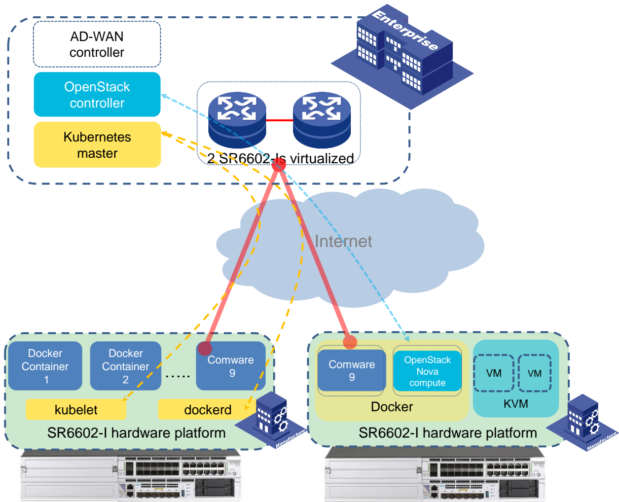
Edge computing solution
